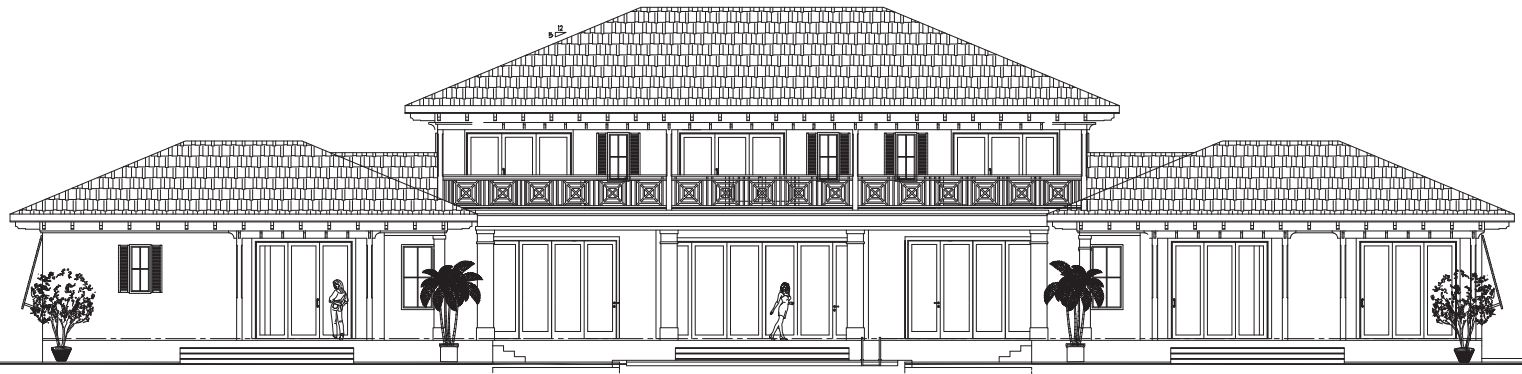
NORTHEAST ELEVATION
